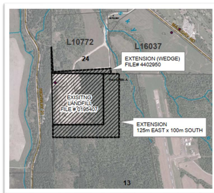
Figure 6-2: Creston Proposed Landfill Extensions
